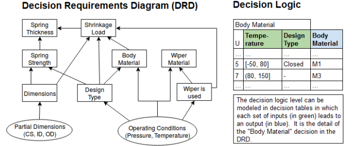
Figure 1. DRD and decision table extract for component design.
